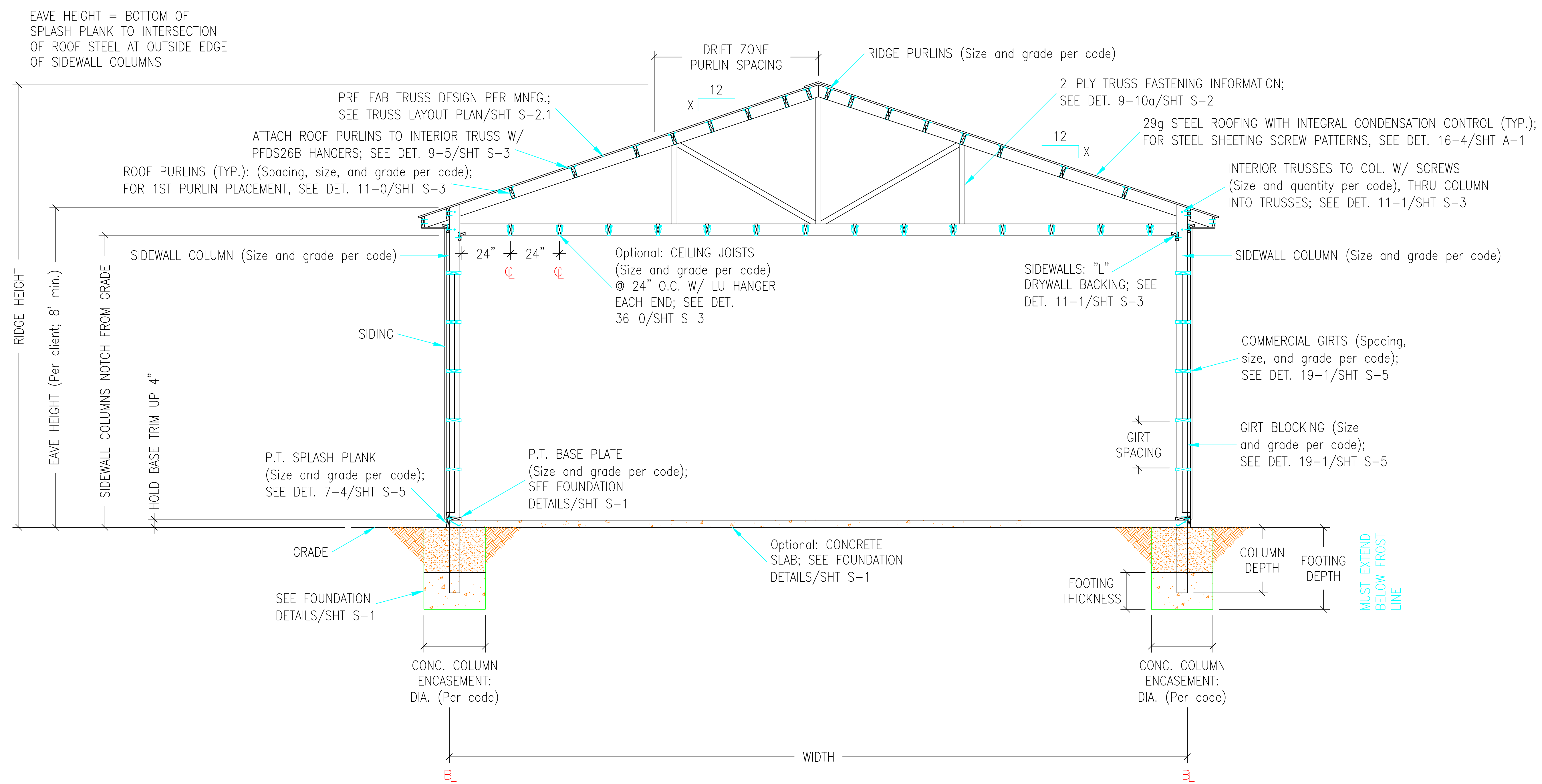
BB BUILDING SECTION S-3 SCALE: 1/4"=1'-0"
